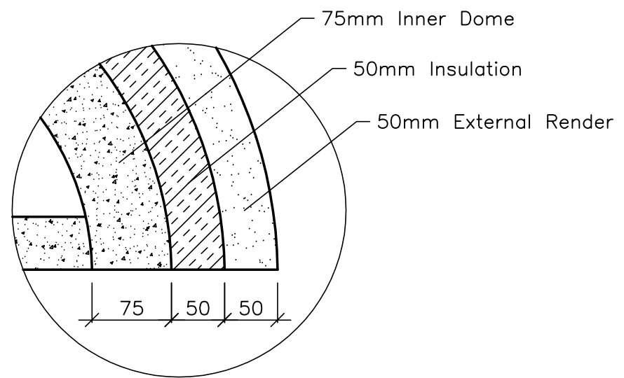
Sectional Detail A
